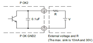
Fig. 3.3 Internal circuit of P OK2 (Open collector method)
