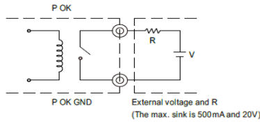
Fig. 3.2 Internal circuit of P OK (Relay, total is 10W)
