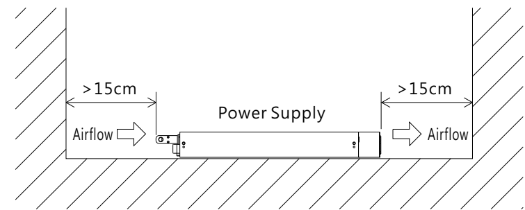
Figure 3-1 Mounting Diagram
