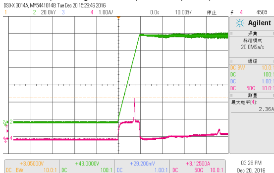
INPUT=110VDC @ FULL LOAD
